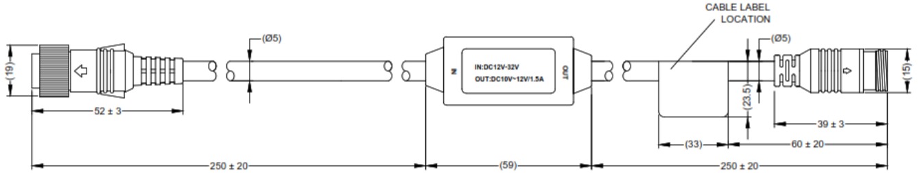
Drawing of AC-24-12 (001) shown. Connectors vary per product, please see table below.
